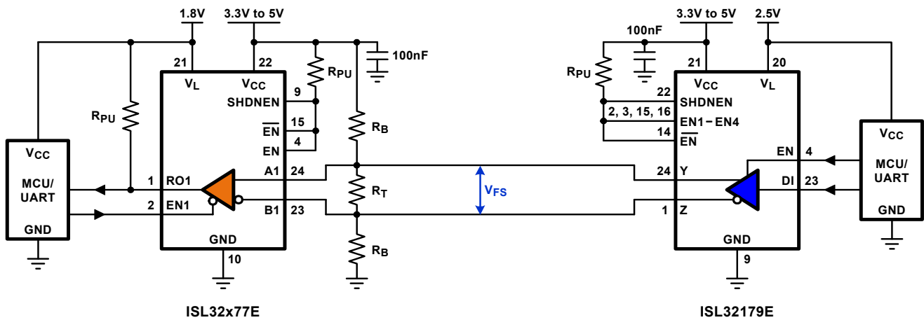
FIGURE 4. NETWORK USING PAIRED ENABLES
