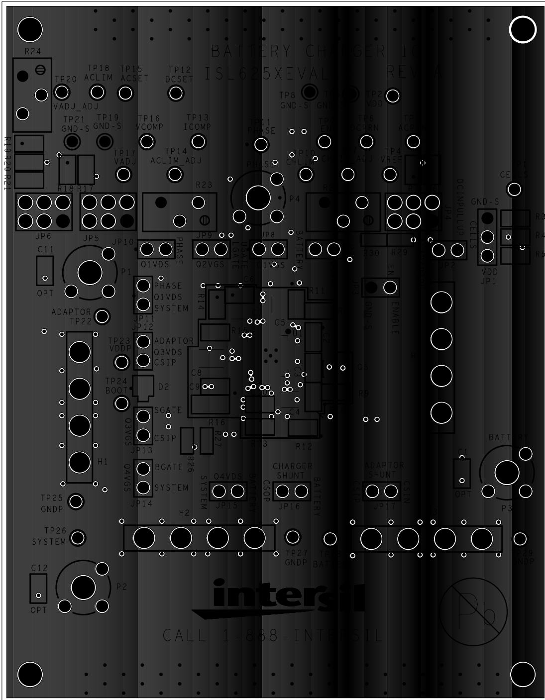
FIGURE 3. LAYER 2 GROUND
