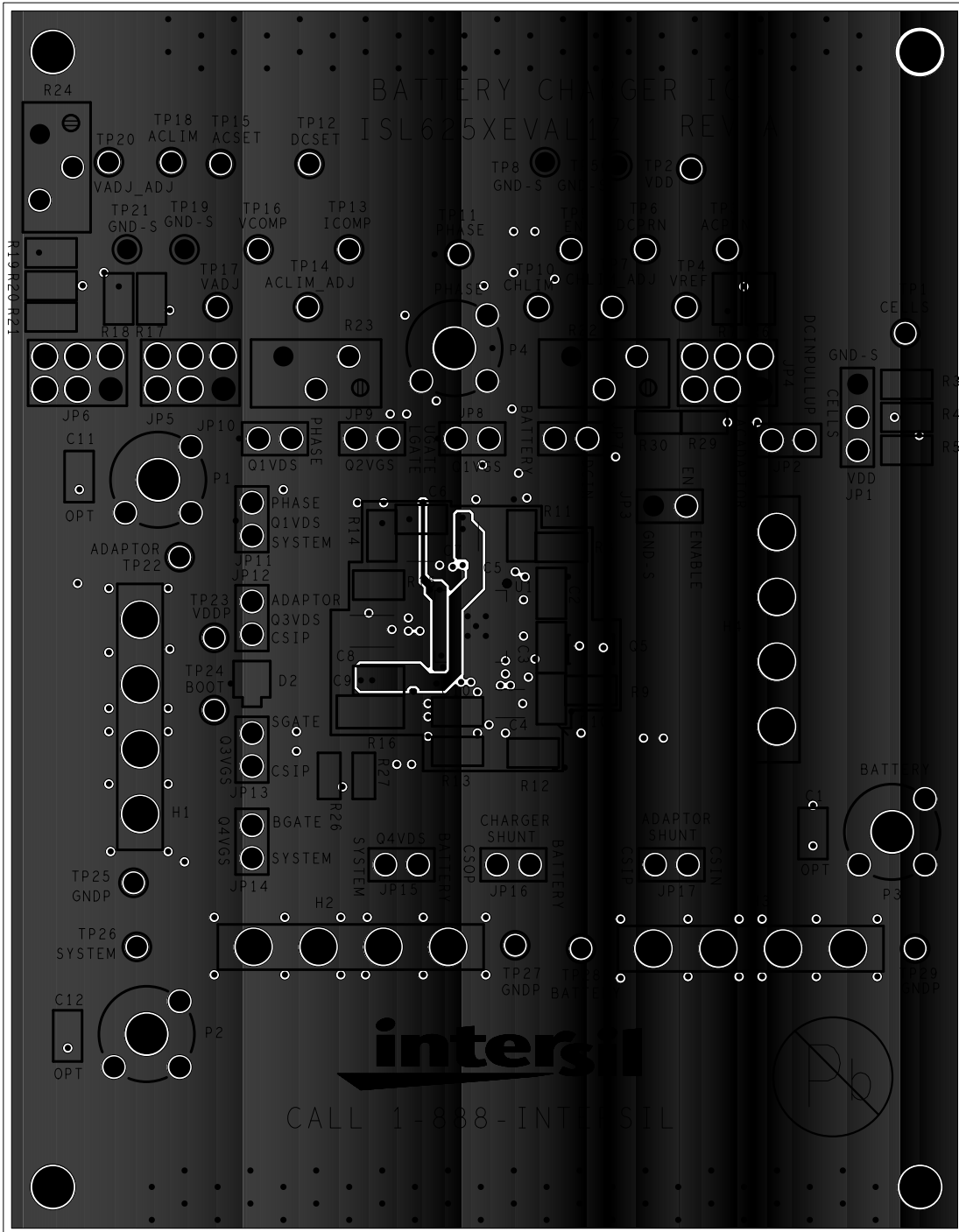
FIGURE 5. LAYER 4 GROUND
