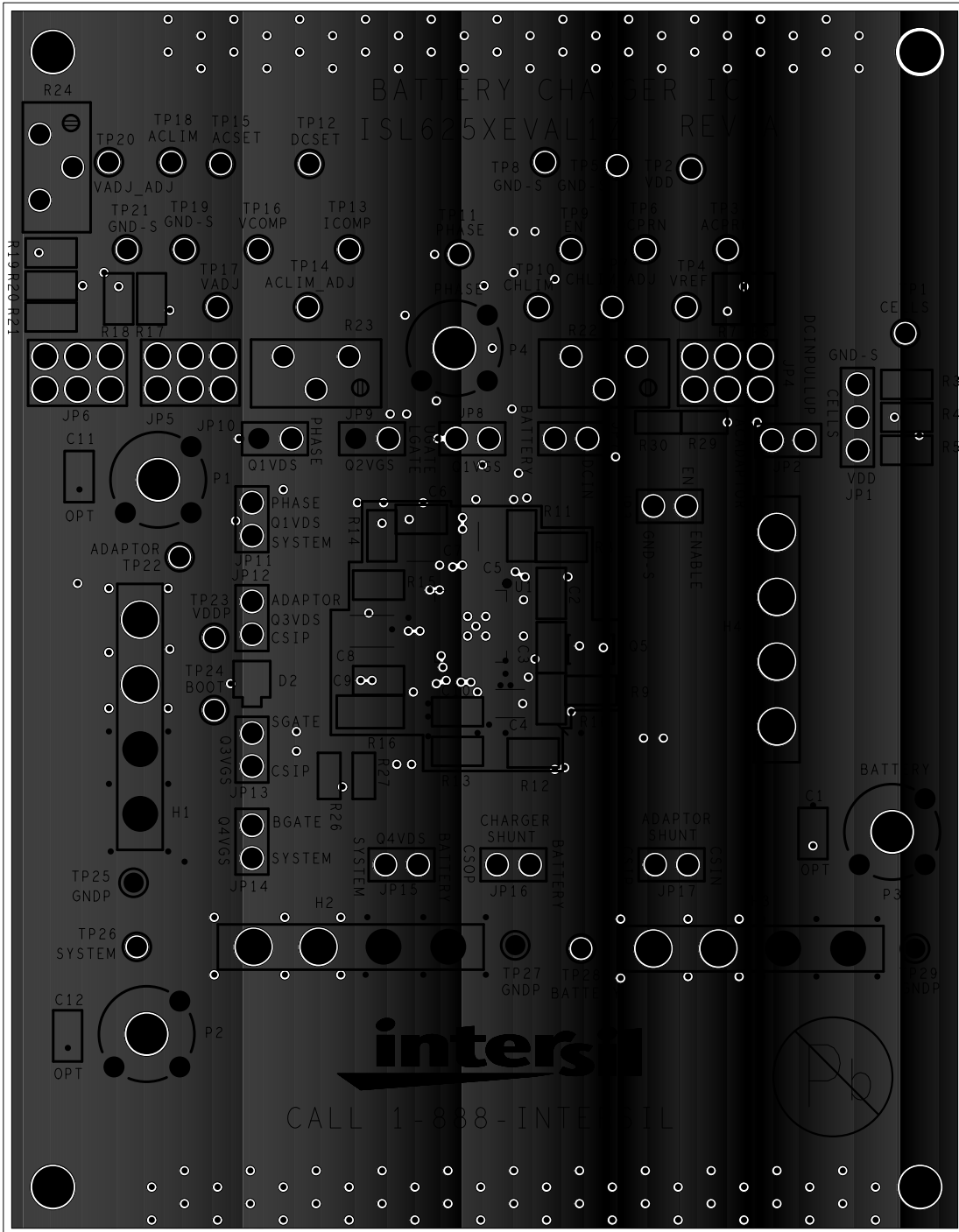
FIGURE 6. LAYER 5 GROUND
