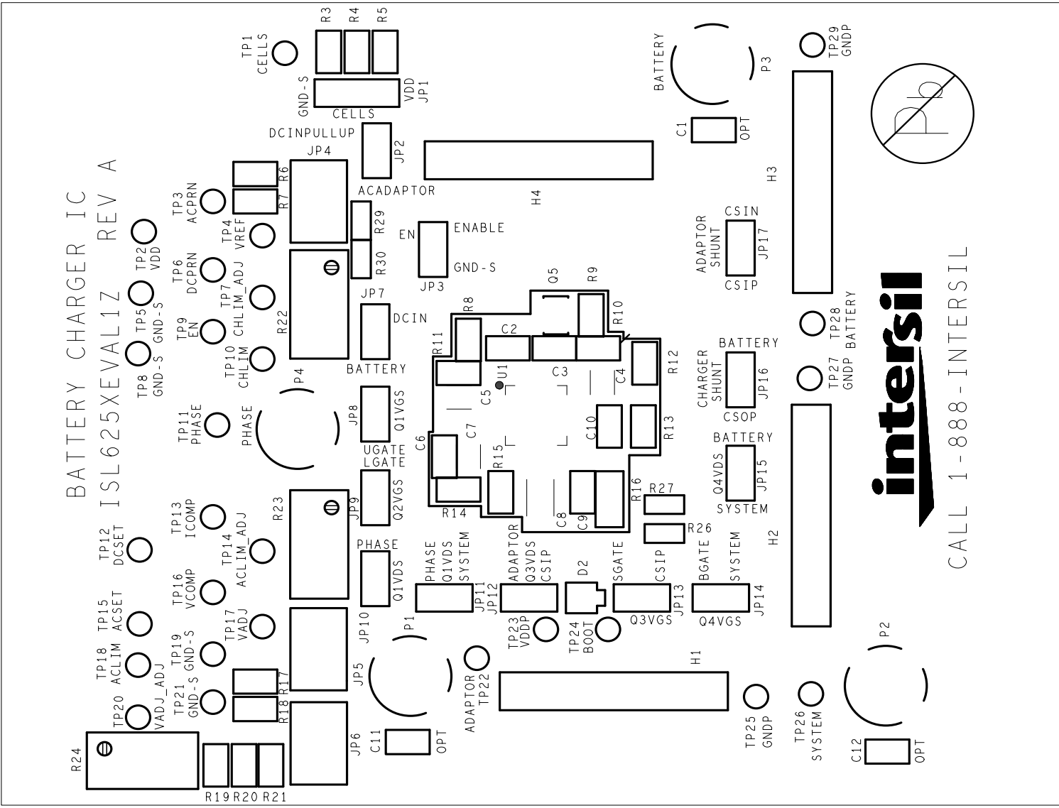
FIGURE 1. TOP SILK
