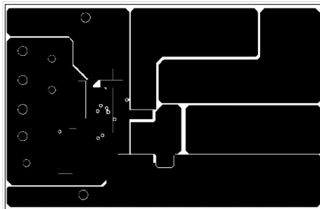
FIGURE 20. ISL6420BEVAL1Z - LAYER 3
