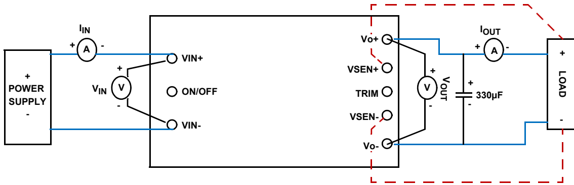
FIGURE 2. CONNECTION DIAGRAM
