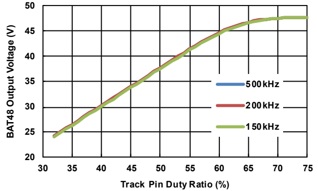
Figure 30. BAT48 Output Voltage at Three Track Pin Frequencies (Digital Tracking Mode, Boost Mode, DE Mode, Phase Drop Disabled, f_{CLK} = 100\text{kHz} )
