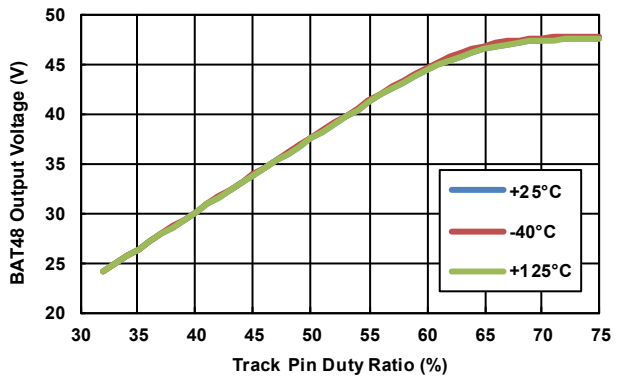
Figure 28. BAT48 Output Voltage (Digital Tracking Mode, FTRK = 200kHz, Boost Mode, DE Mode, Phase Drop Disabled, f_{CLK} = 100\text{kHz} )
