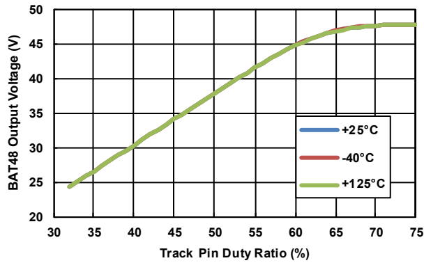
Figure 27. BAT48 Output Voltage (Digital Tracking Mode, FTRK = 500kHz, Boost Mode, DE Mode, Phase Drop Disabled, f_{CLK} = 100\text{kHz} )
