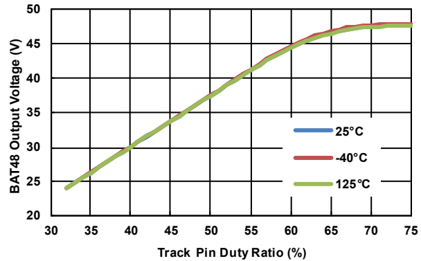
Figure 29. BAT48 Output Voltage (Digital Tracking Mode, FTRK = 150kHz, Boost Mode, DE Mode, Phase Drop Disabled, f_{CLK} = 100\text{kHz} )
