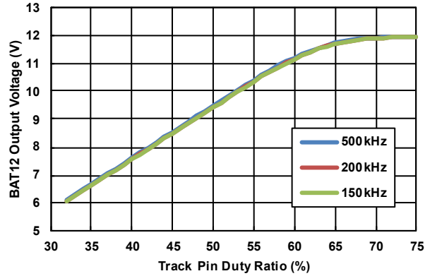
Figure 26. BAT12 Output Voltage at Three Track Pin Frequencies (Digital Tracking Mode, Buck Mode, DE Mode, Phase Drop Disabled, f_{CLK} = 100\text{kHz} )
