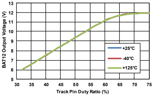
Figure 25. BAT12 Output Voltage (Digital Tracking Mode, FTRK = 150kHz, Buck Mode, DE Mode, Phase Drop Disabled, f_{CLK} = 100\text{kHz} )
