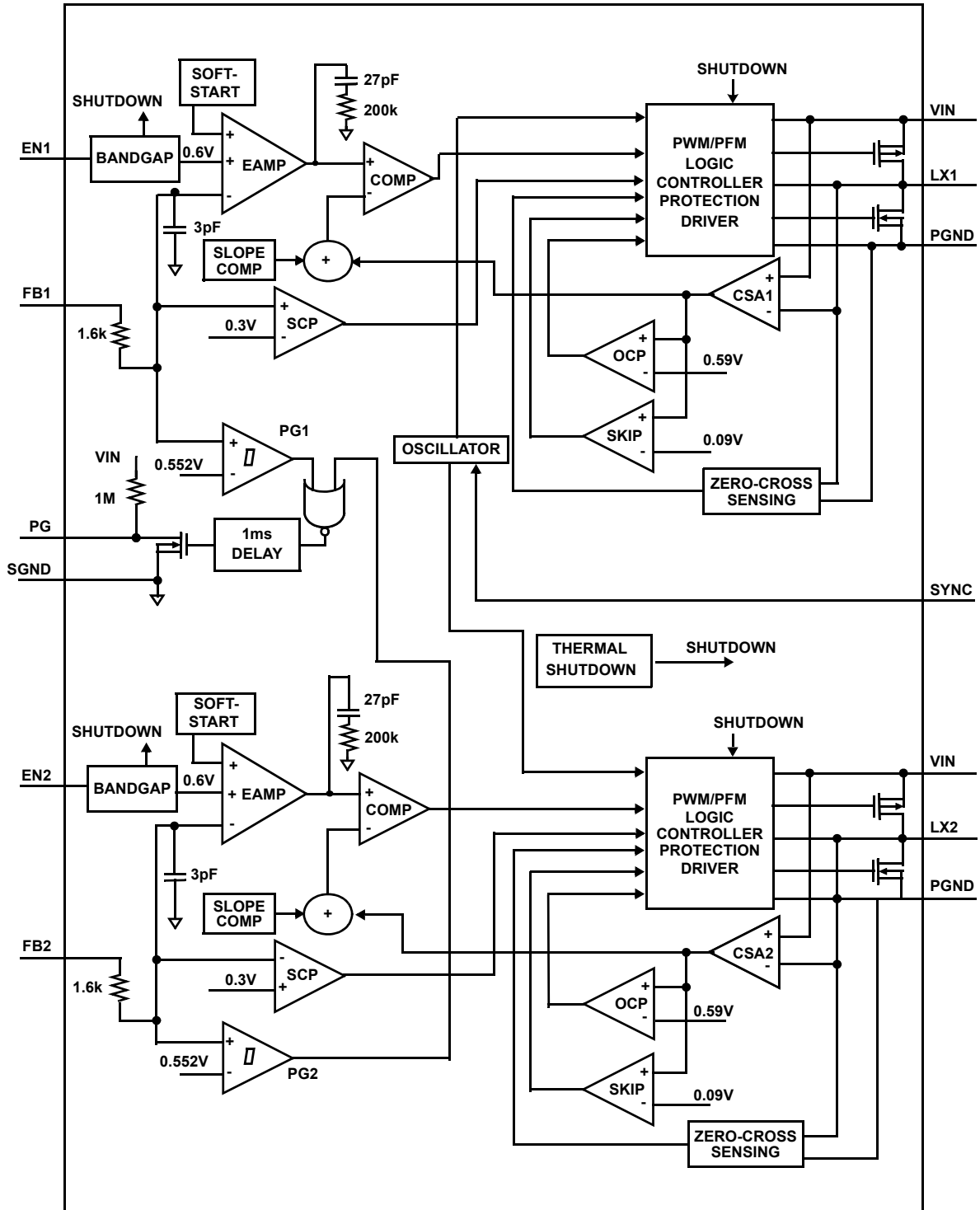
FIGURE 44. BLOCK DIAGRAM
