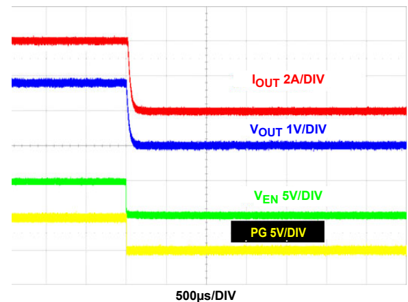
FIGURE 21. SHUTDOWN AT 4A LOAD (PFM)
