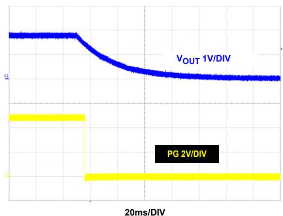
FIGURE 32. OVER-TEMPERATURE PROTECTION
