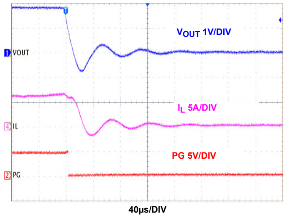
FIGURE 30. OVERCURRENT PROTECTION
