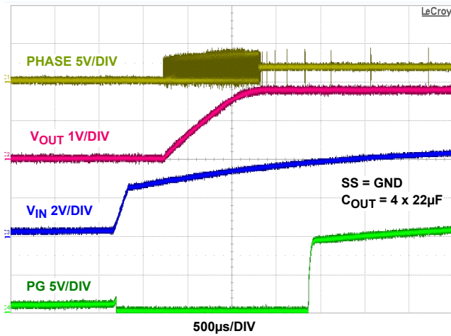
FIGURE 17. V_{\text{IN}} START-UP AT NO LOAD ( \text{SYNC} = \text{GND} )
