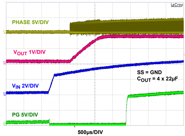
FIGURE 18. V_{\text{IN}} START-UP AT NO LOAD ( \text{SYNC} = V_{\text{DD}} )
