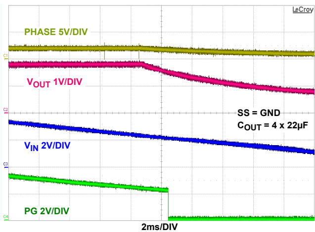
FIGURE 21. V_{\text{IN}} SHUTDOWN AT NO LOAD ( \text{SYNC} = \text{GND} )
