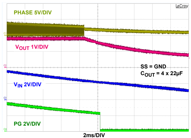
FIGURE 22. V_{\text{IN}} SHUTDOWN AT NO LOAD ( \text{SYNC} = V_{\text{DD}} )
