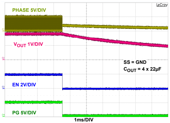
FIGURE 20. EN SHUTDOWN AT NO LOAD ( \text{SYNC} = V_{\text{DD}} )
