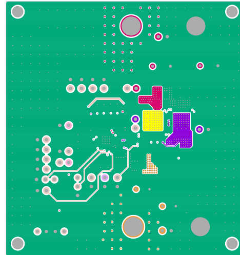
FIGURE 8. LAYER 3
