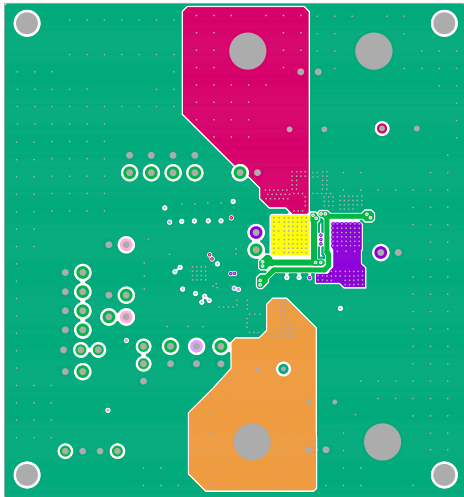
FIGURE 7. LAYER 2
