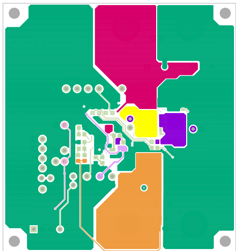
FIGURE 9. BOTTOM LAYER
