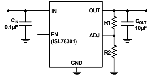
FIGURE 12. ADJUSTABLE VERSION
