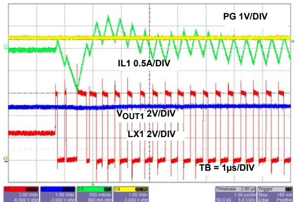
FIGURE 30. RECOVERY FROM HARD SHORT NEGATIVE CURRENT WAVEFORMS V_{OUT1} CHANNEL 1
