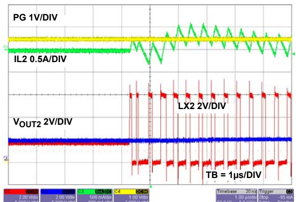
FIGURE 32. RECOVERY FROM HARD SHORT NEGATIVE CURRENT WAVEFORMS V_{OUT2} CHANNEL 2
