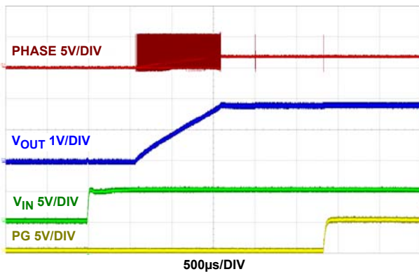
FIGURE 26. START-UP V_{IN} AT NO LOAD (ISL80031A) f_{SW} = 2\text{MHz} , V_{IN} = 5\text{V} , PFM, T_A = +25^\circ\text{C}
