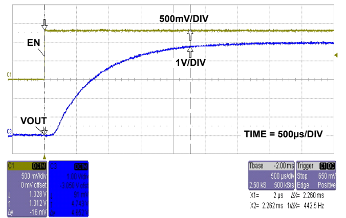
FIGURE 8. START-UP WAVEFORM
