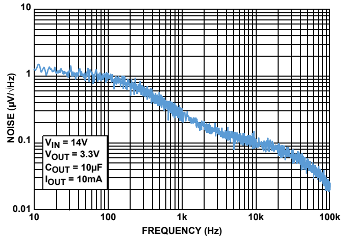
BW = 100 < f < 100kHz output noise voltage ~ 26 \mu V_{rms} FIGURE 12. OUTPUT NOISE SPECTRAL DENSITY, I_{OUT} = 10mA
