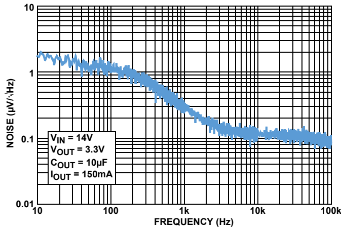
BW = 100 < f < 100kHz output noise voltage ~ 38 \mu V_{rms} FIGURE 13. OUTPUT NOISE SPECTRAL DENSITY, I_{OUT} = 150mA
