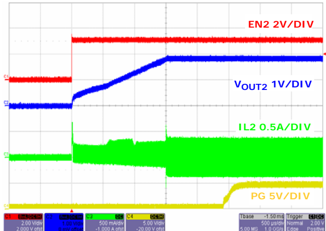
FIGURE 19. SOFT-START WITH NO LOAD CHANNEL 2
