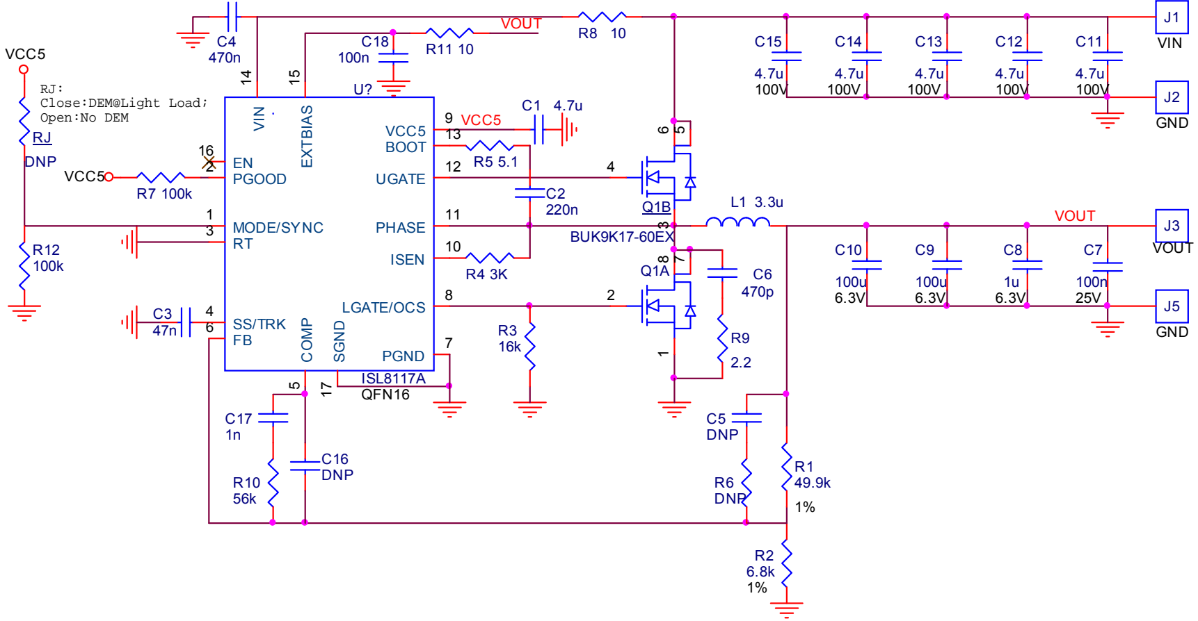
Figure 6. ISL8117ADEMO3Z Schematic
