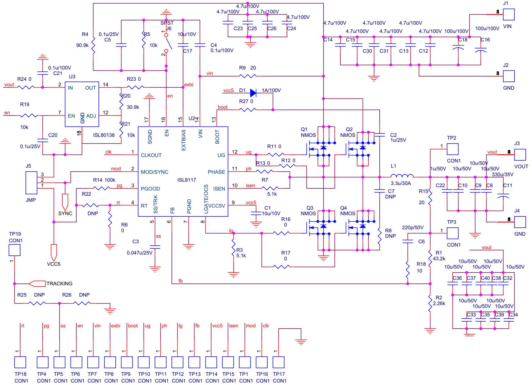
FIGURE 20. ISL8117EVAL2Z SCHEMATIC
