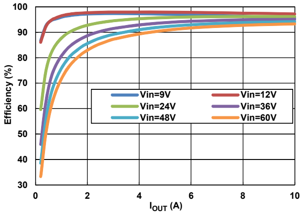
Figure 14. Efficiency, CCM
