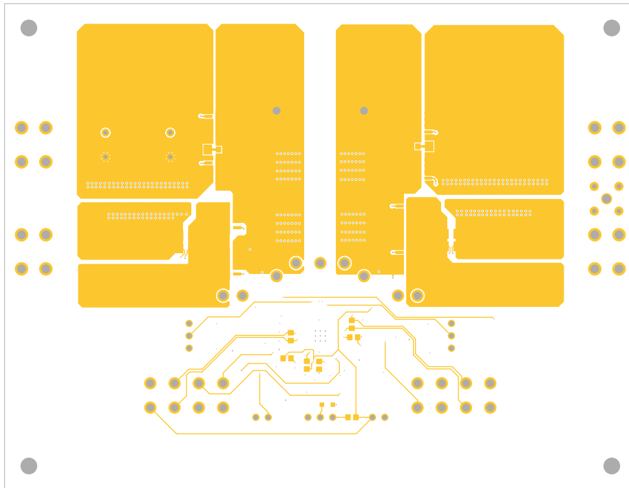
Figure 12. Bottom Layer
