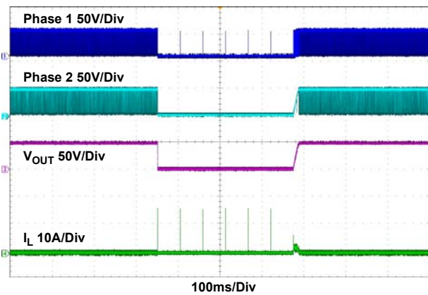
Figure 27. Short-Circuit Waveform
