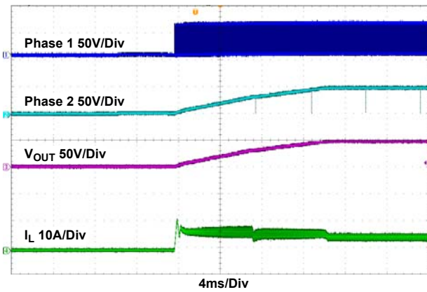
Figure 26. Start-Up Waveform, V_{IN} = 60V , I_{OUT} = 5A , CCM
