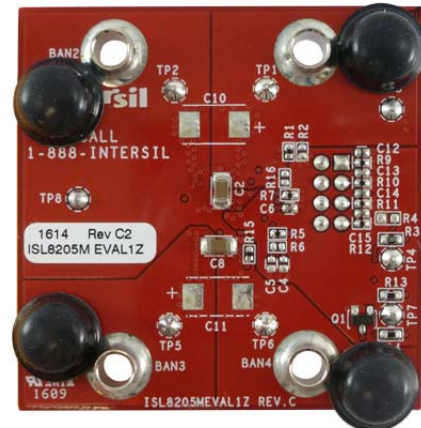
FIGURE 3. BOTTOM OF BOARD
