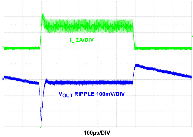
FIGURE 34. LOAD TRANSIENT (DCM)
