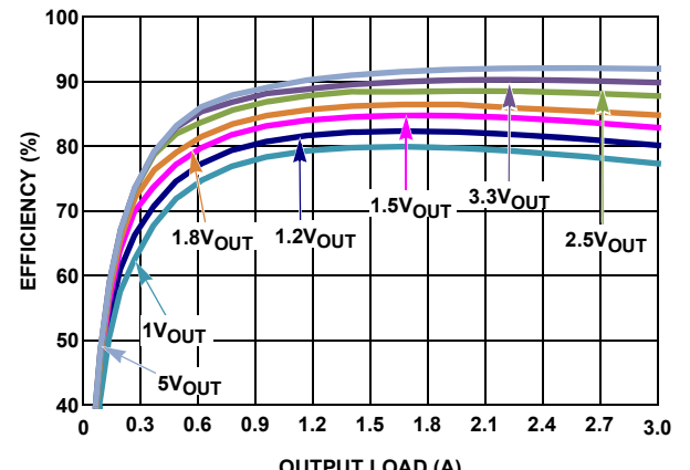
FIGURE 8. EFFICIENCY vs LOAD, 18V IN CCM
