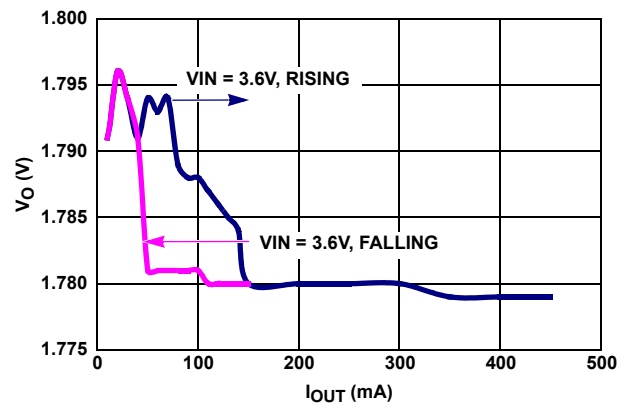
FIGURE 4. OUTPUT VOLTAGE vs LOAD CURRENT (ISL9103, V_{O\_NORMAL} = 1.8\text{V} )
