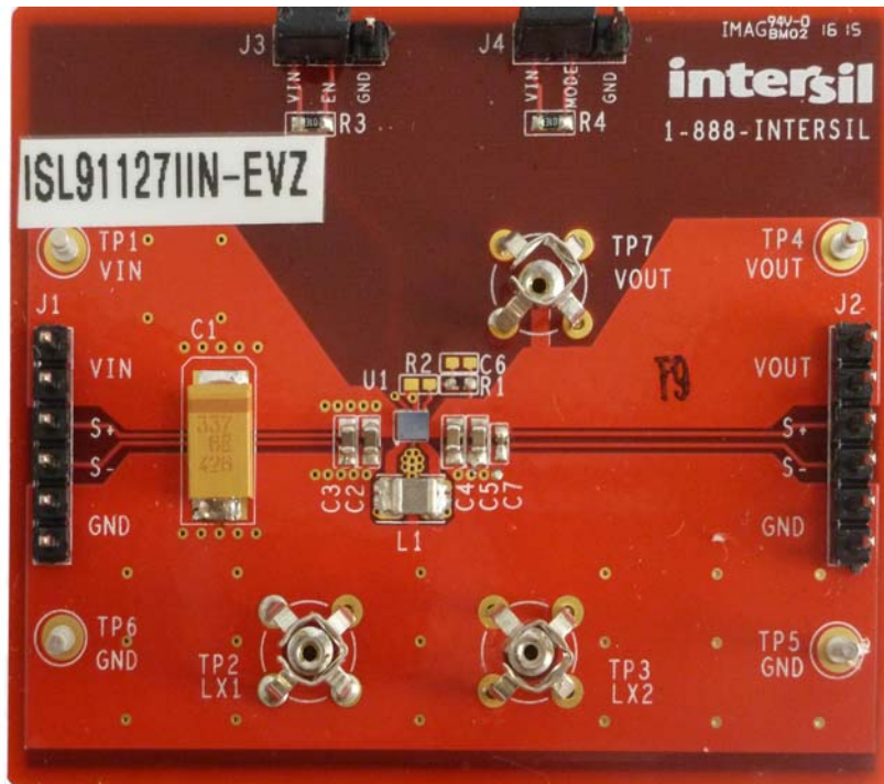
FIGURE 5. ISL91127IIN-EVZ BOARD
