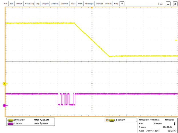
Figure 18. 1.1V to 0.5V DVS; Load = 5A, Slew Rate = 3mV/μs
