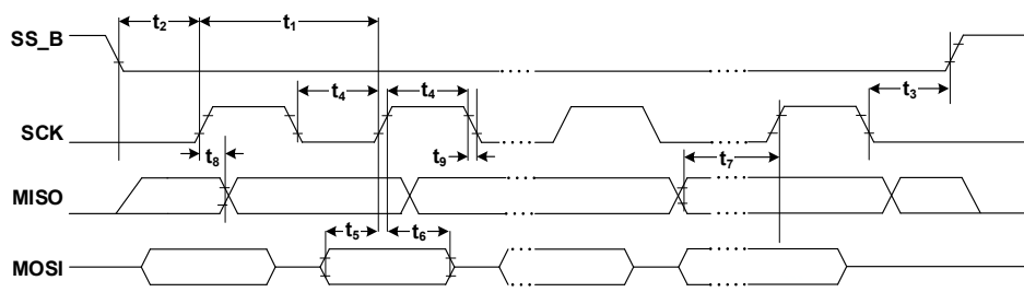
Figure 30. SPI Timing for IO_SPICPHA = 0, IO_SPICPOL = 0
