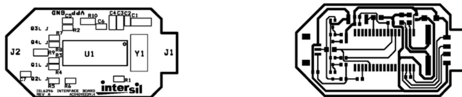
FIGURE 22. LAYOUT OF THE USB-TO-XSD INTERFACE BOARD
