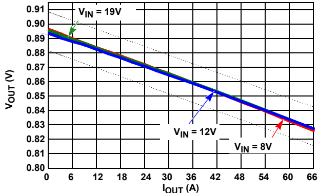
FIGURE 1. LOAD LINE REGULATION
