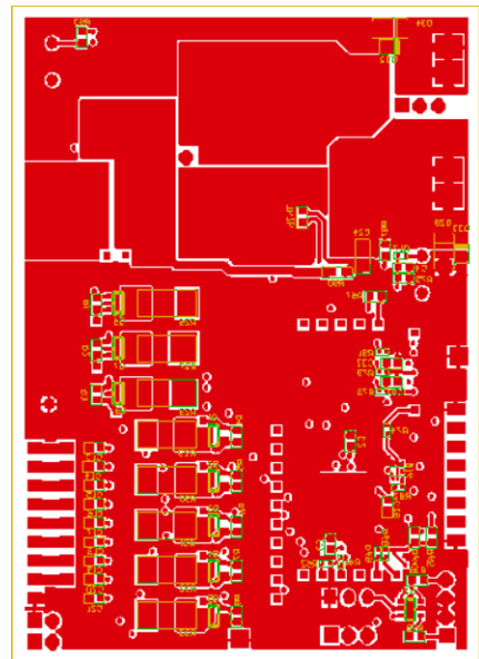
FIGURE 55. BOTTOM LAYER
