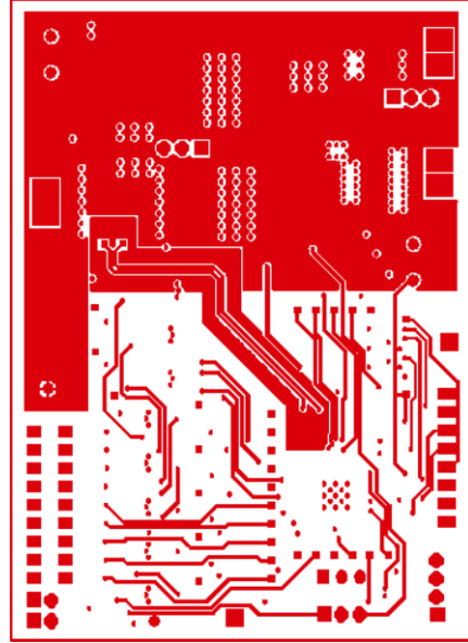
FIGURE 53. MIDDLE LAYER 1
