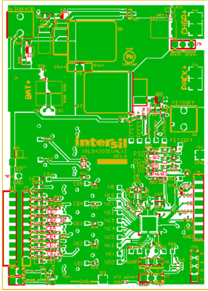
FIGURE 52. TOP LAYER
