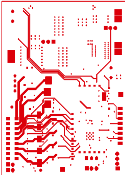
FIGURE 54. MIDDLE LAYER 2
