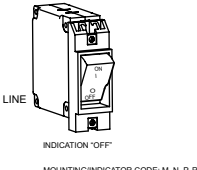
MARKING DETAIL "B" (SEE TABLE)
