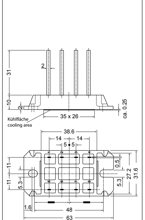
X105 V1-B-Pack Weight = 30 g a: pin length = 31 mm b: pin length = 16 mm
