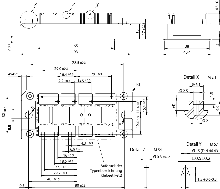
X104 V2-Pack Weight = 76 g See data sheet for pin arrangement
