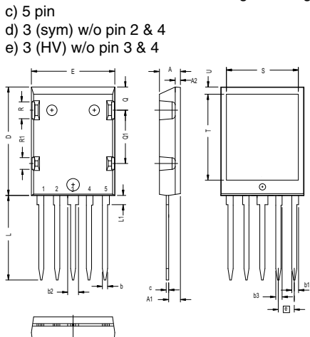
XO22 ISOPLUS264™ Weight = 7.5 g
