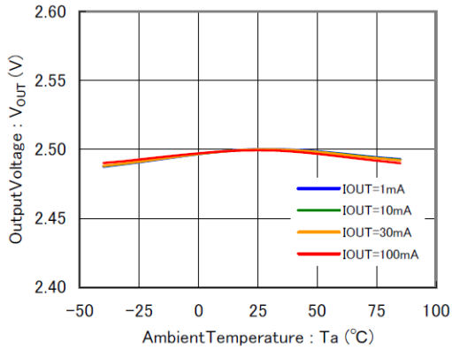
IXD1421 V IN = V OUT + 1.0 V
