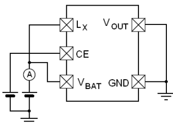
Circuit ④
