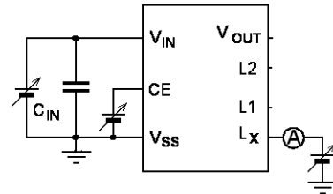
Circuit ⑧
