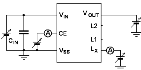
Circuit ⑤
