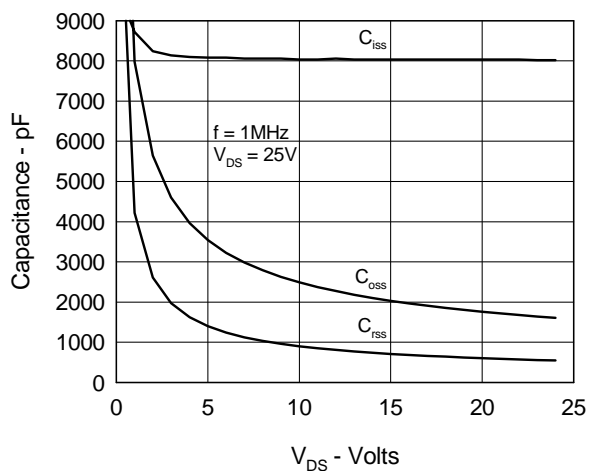
Fig.8 Capacitance Curves
