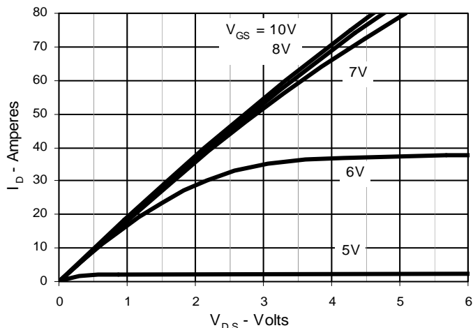
Fig. 3. Output Characteristics
