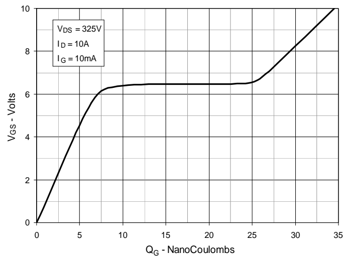
Fig. 11. Gate Charge
