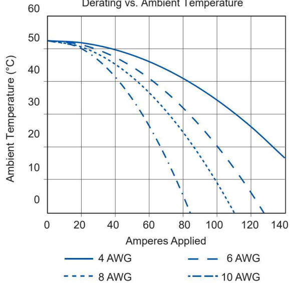
SBS®X-75A Primary Contacts Only Derating vs. Ambient Temperature
