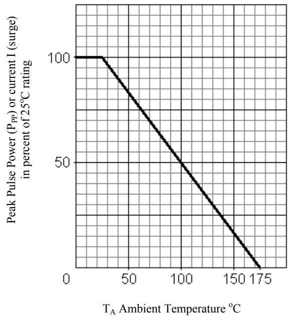
FIG. 4 Derating Curve
