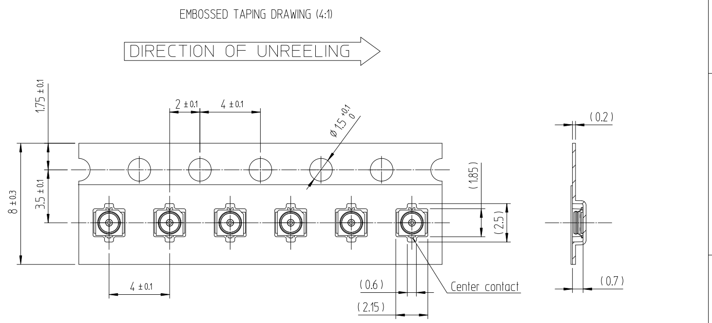
REEL DRAWING(FREE)
