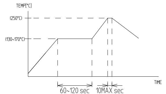
RECOMMENDED REFLOW TEMPERATURE PROFILE
