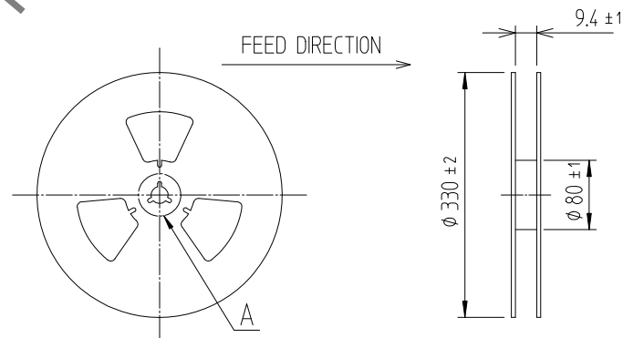
DETAIL 'A'(FREE)
