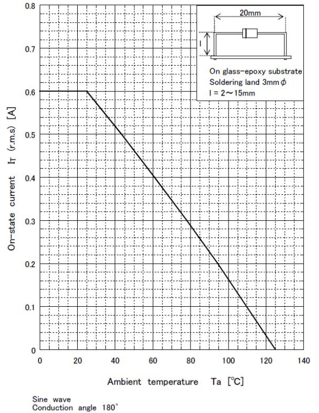
Derating curve
