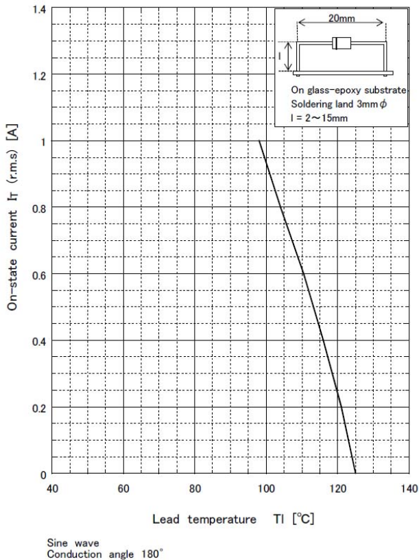
Derating curve
