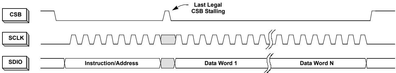
Figure 41. N-Byte Transfer
