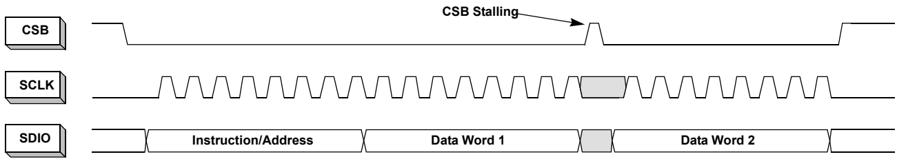
Figure 40. 2-Byte Transfer
