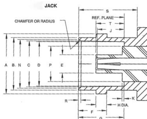
Dimensions in inches with metric equivalents (mm) in parentheses.
