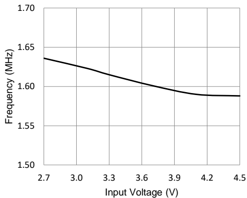
Step-up Converter Switching Frequency
