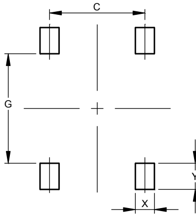
T-DFN5564-4
