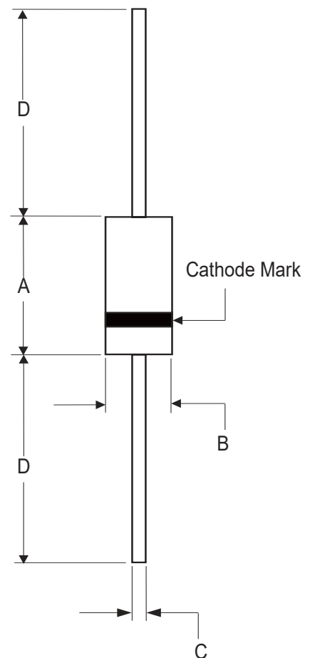
DO-201AE
