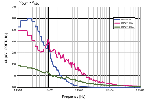
Figure 30. Noise spectrum vs. frequency (V OUT = V ADJ )
