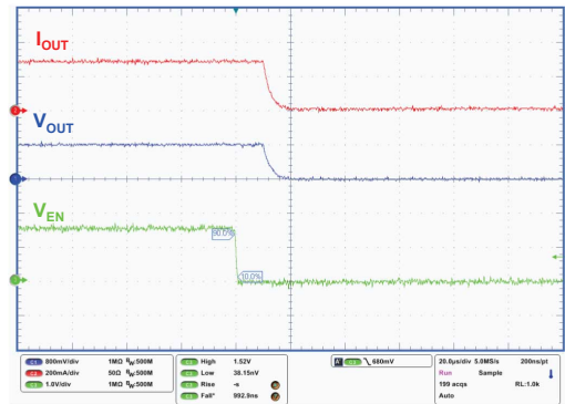
Figure 36. Turn-off by enable
