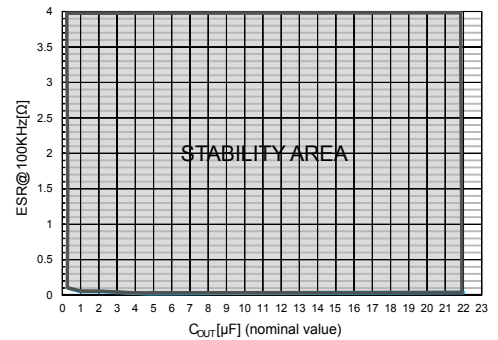
Figure 32. Stability plan vs. (C OUT , ESR)
