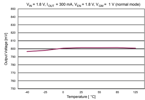
Figure 6. Output voltage vs. temperature ( V_{IN} = 1.8 \text{ V} , I_{OUT} = 300 \text{ mA} , normal mode)
