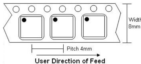
Figure 55. DFN6 reel oriented
