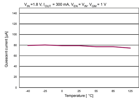
Figure 16. Quiescent current vs. temperature ( I_{OUT} = 300 mA, normal mode)
