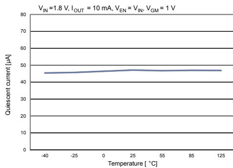
Figure 15. Quiescent current vs. temperature ( I_{OUT} = 10 mA, normal mode)
