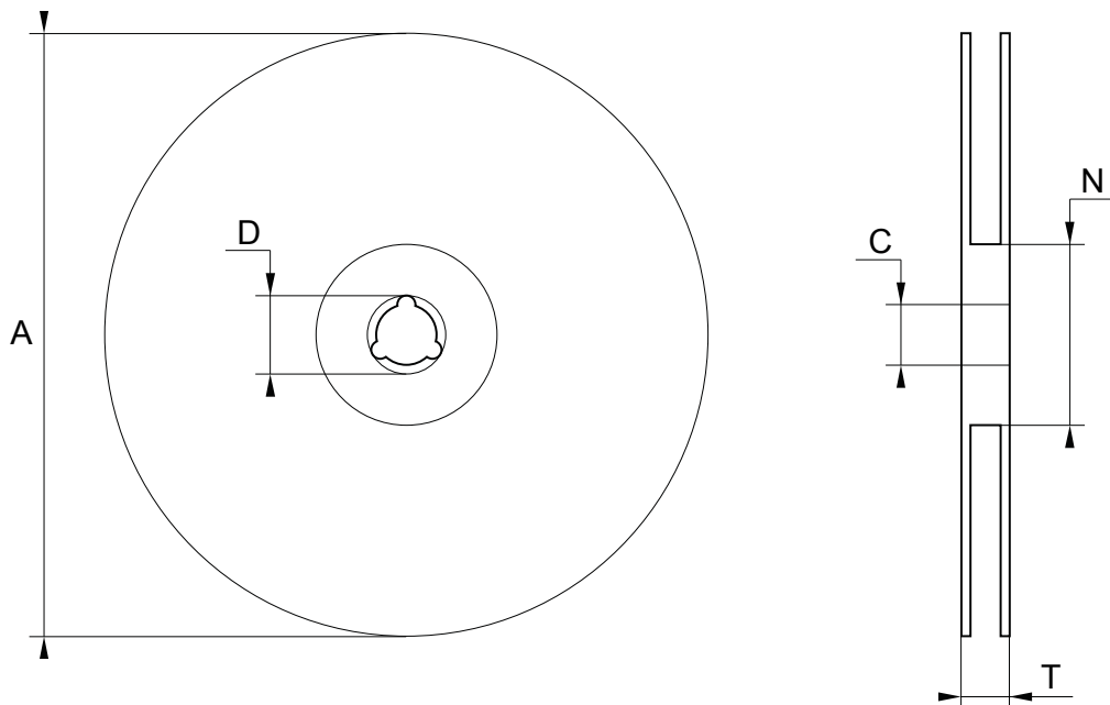
Figure 56. Reel outline
