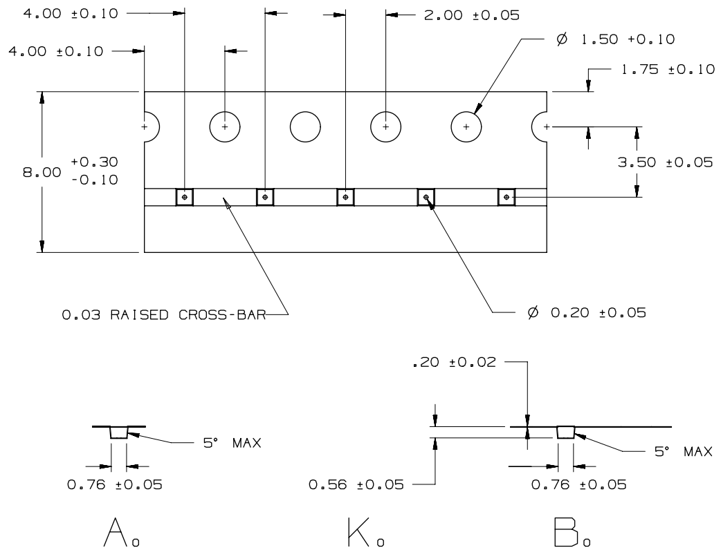
Figure 51. Flip-chip 4 tape
