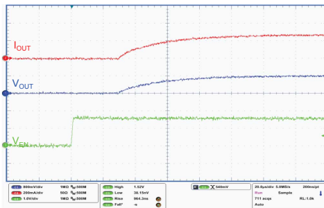
Figure 37. Startup by enable ( I_{OUT} = 300\text{ mA} , normal mode)
