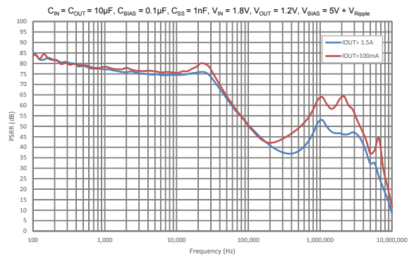
Figure 13. V_{BIAS} PSRR vs. frequency ( V_{IN} = 1.8 V, V_{OUT} = 1.2 V)
