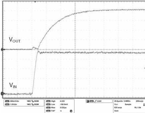
Figure 30. Startup transient
